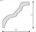
TI NOMASTYL® H 140 x W 140 mm
