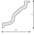
N24 NOMASTYL® H 70 x W 20 mm r 180 mm
